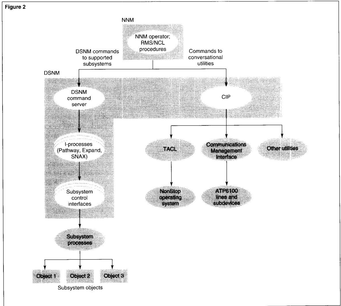
Figure 2. DSNM command server and CIP under NNM.
