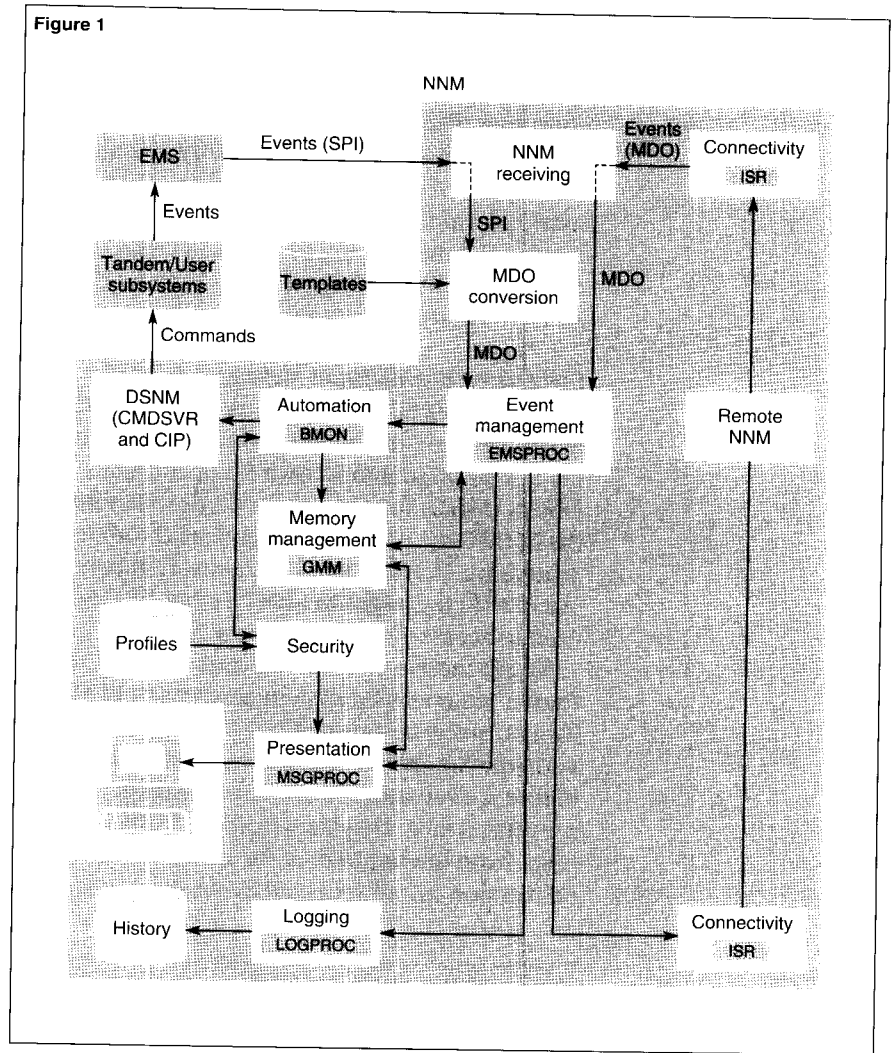
Figure 1. Design of NNM event management functions.
