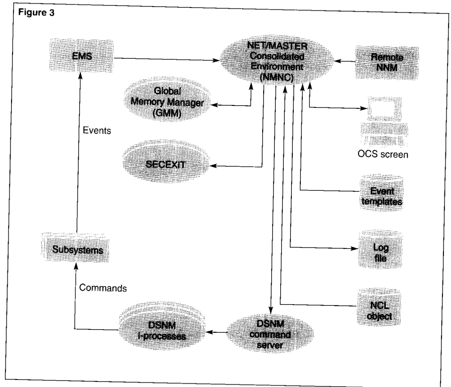
Figure 3. NNM basic configuration mode.
